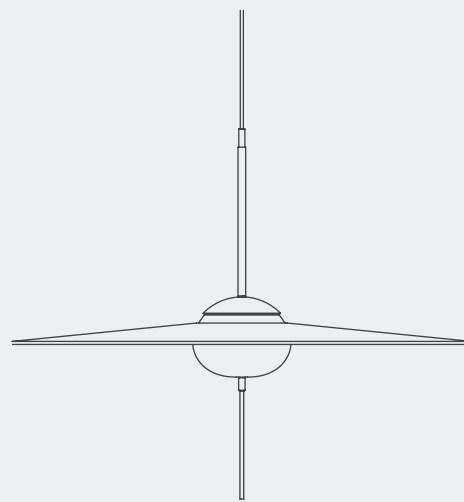
MONO L600 Glass planet Ø128 mm Tilting glass ring Ø600 mm
