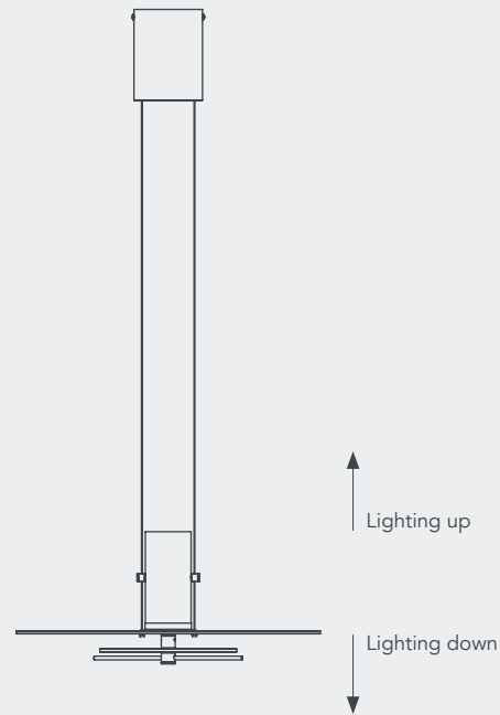
DELUMINA PENDANT Glassing ring Ø400mm
